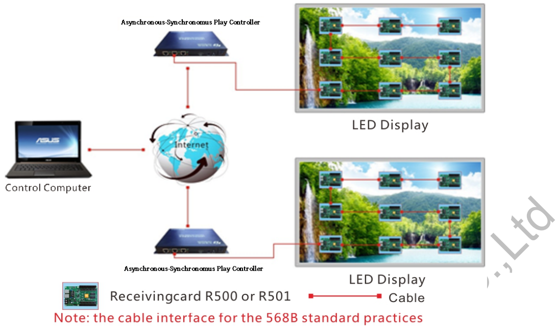
1-1 Asynchronous cluster management mode
