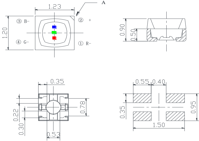
参考焊盘 Reference Soldering Pad
